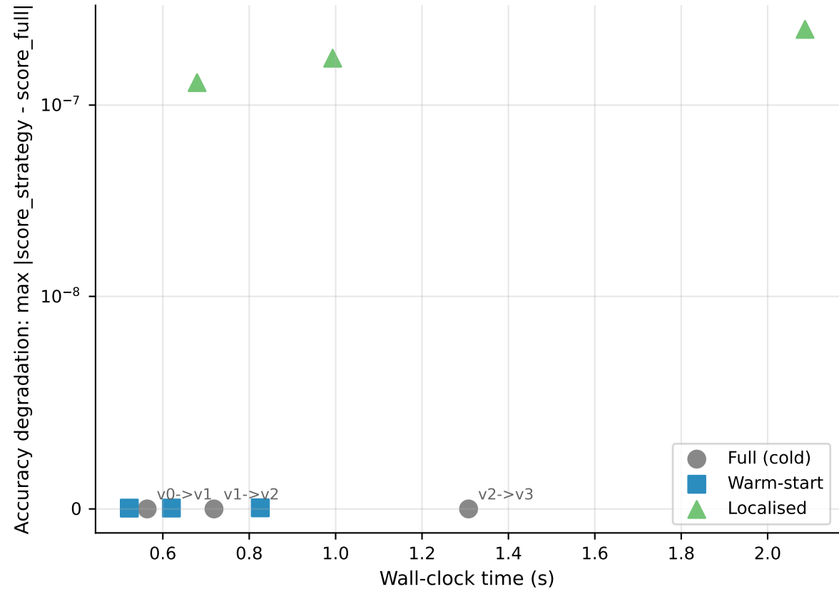
Group C - Cost vs Accuracy Trade-off
